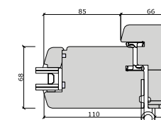
Double Handle
