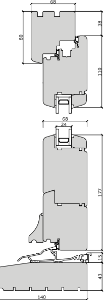
Contemporary Lipped Open In
