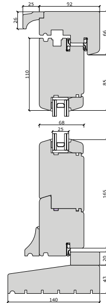
Contemporary Flush Open Out
