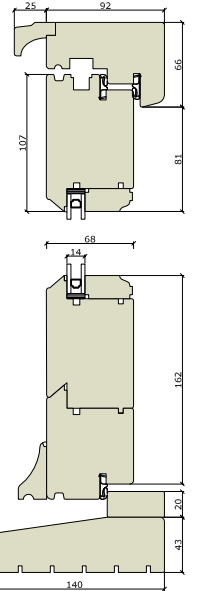
Heritage Flush Open Out
