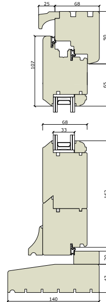
Traditional Lipped Open Out
