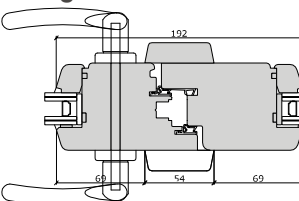
Single Handle
