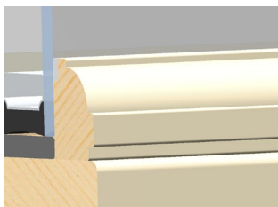
Traditional Internal
