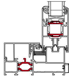
BSC94 Mono Rail – Cill
